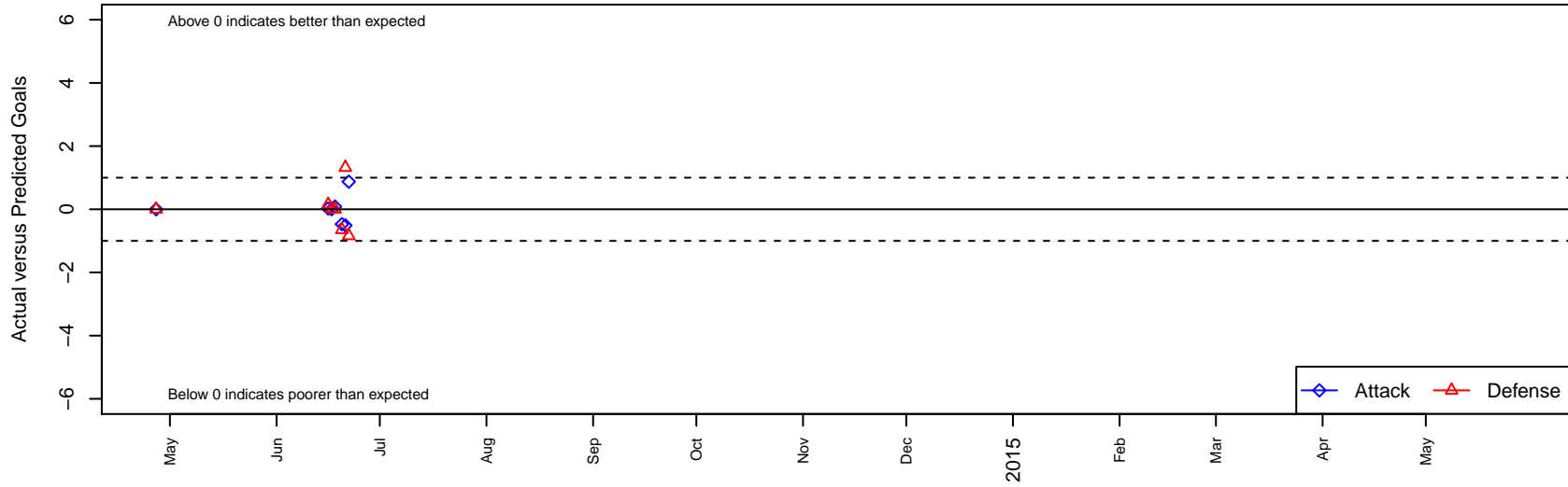
Santa Barbara SC White B95 Dots are actual minus expected GF (blue circles) and GA (red triangles). Blue line is smoothed change in attack strength. Red is smoothed change in defense strength.
